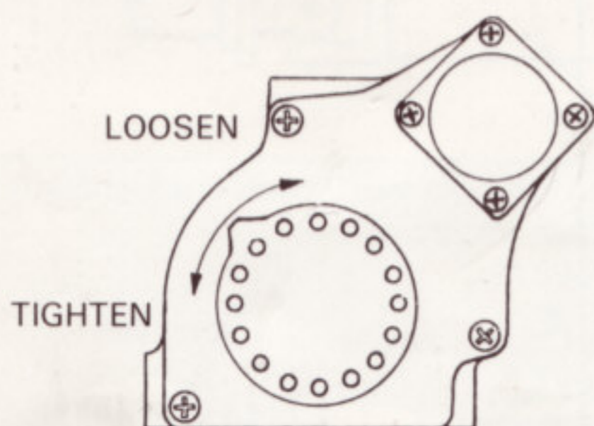
BELT TENSION ADJUSTMENT
