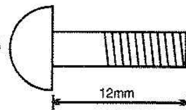
3X12mm SHOULDER SCREW
