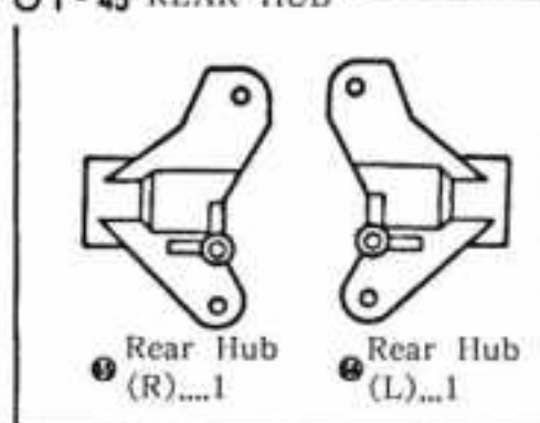
OT-45 REAR HUB
