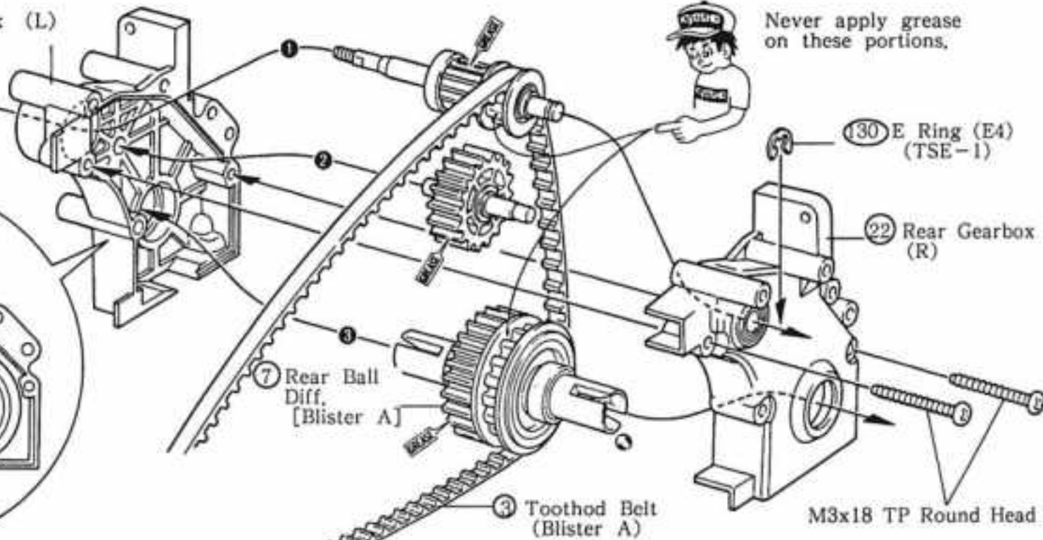
[Assemble View]
