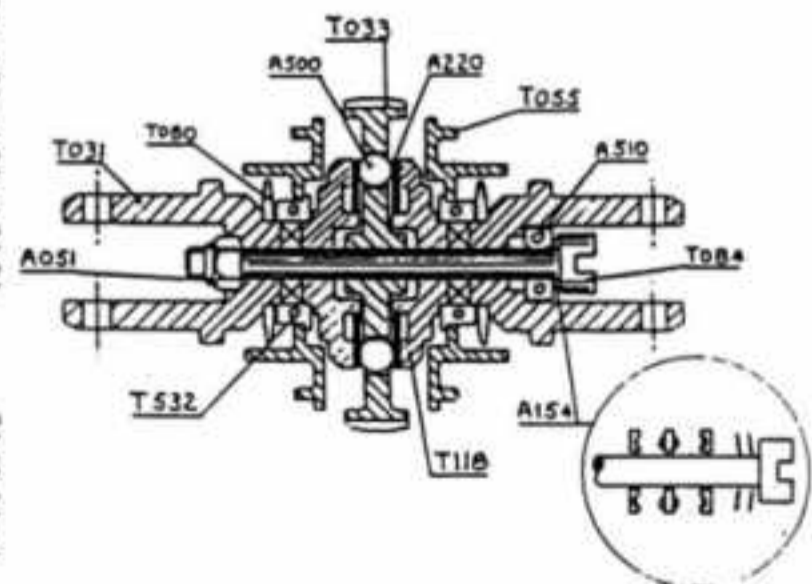
CROSS SECTION THROUGH DIFFERENTIAL
