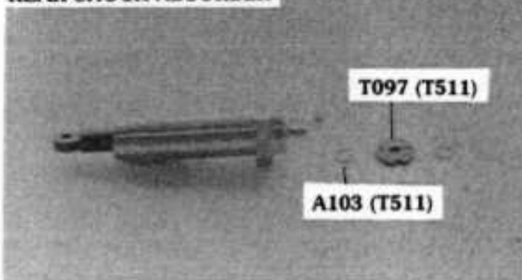
A103 'E' clip 1/8" x .012" T097 Piston 2sq. mm hole (rear)
