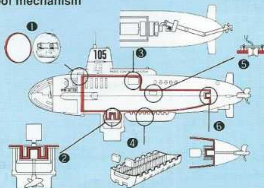
Exploration submarine water proof mechanism
